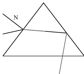
Figura 1.3: Prisma
