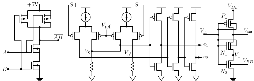
Figura 1.11: Porta Nand CMOS
