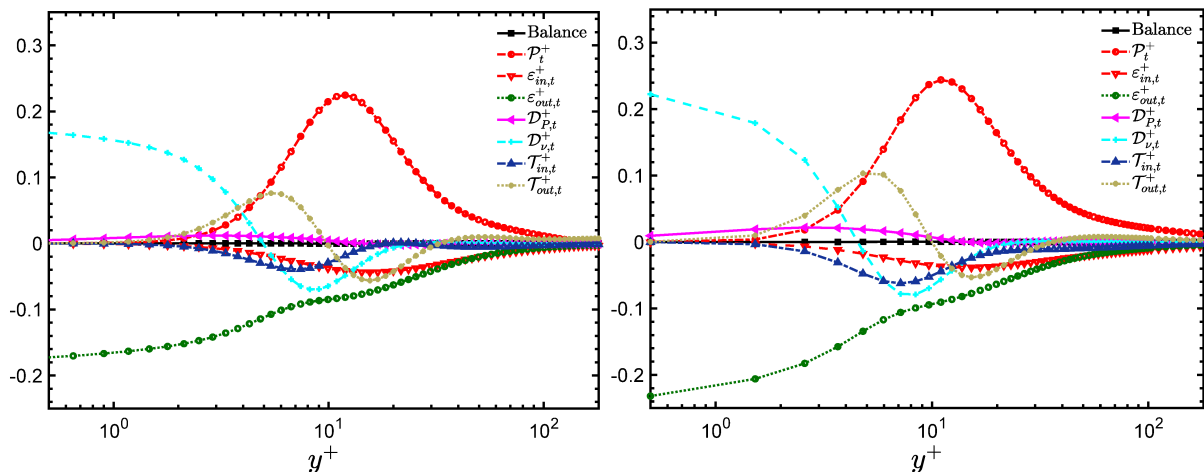
Figure 3.13 – Turbulent kinetic energy budget (Eq. 2.35) at Re_\tau = 180 and 1000, respectively.
