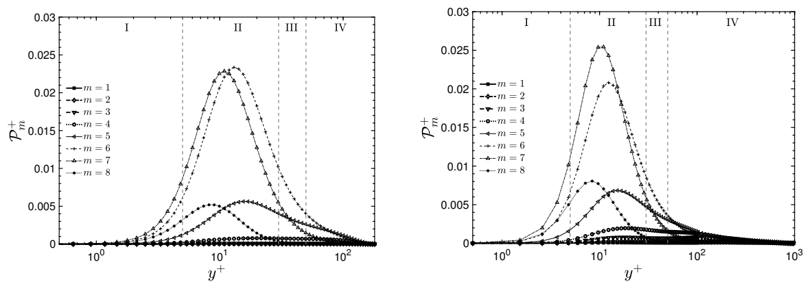
Figure 3.31 – Band distribution for turbulent production for various wavenumber bins, P_m^+ , vs. distance to the wall, y^+ , at Re_\tau = 180 and 1000 , respectively.
