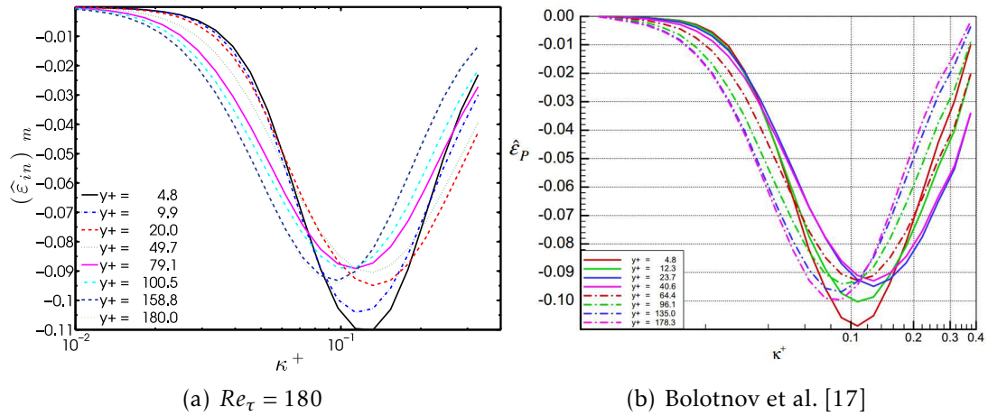
Figure B.7 – In-plane dissipation spectra \epsilon_{in}^+ at various y^+ locations.
