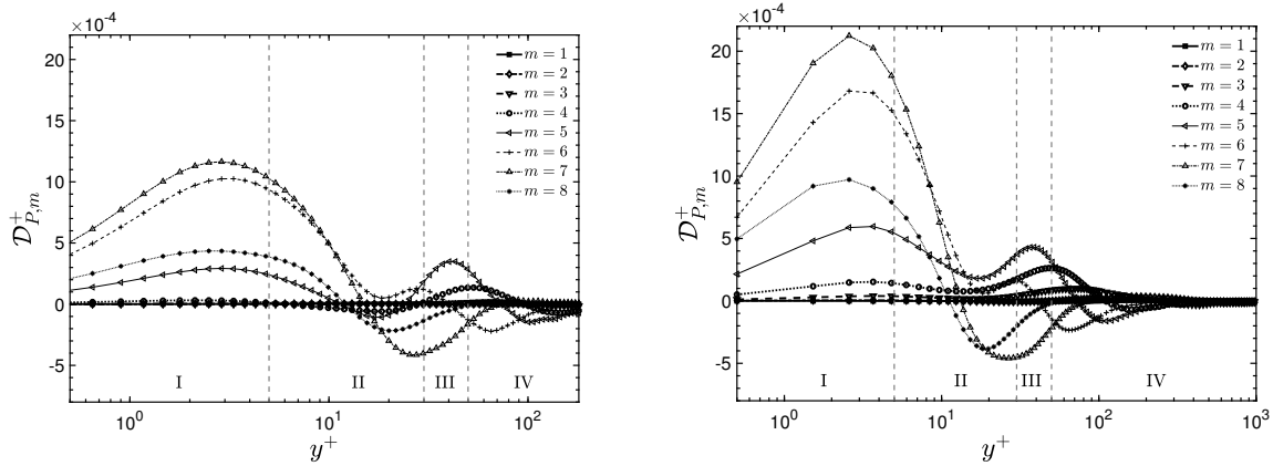
Figure 3.37 – Band distribution for pressure diffusion for various wavenumber bins, D_{P,m}^+ vs. distance to the wall, y^+ , at Re_\tau = 180 and 1000 , respectively.
