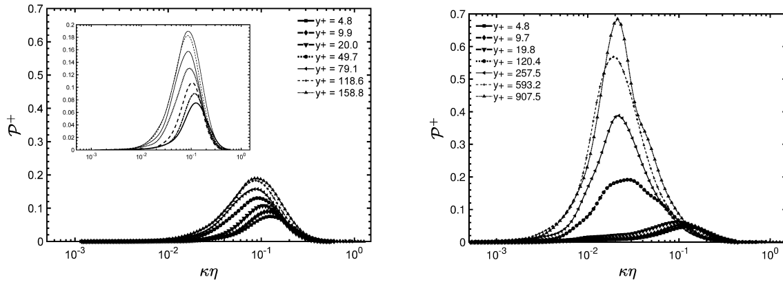
Figure 3.19 – Turbulent production spectral density, \mathcal{P}^+ , at various y^+ location at Re_\tau = 180 and 1000 , respectively.
