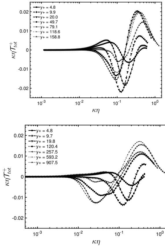
Figure 3.26 – Total nonlinear transfer spectral density, \kappa\eta\mathcal{T}_{tot}^+ , at various y^+ locations at Re_\tau = 180 and 1000 , respectively.
