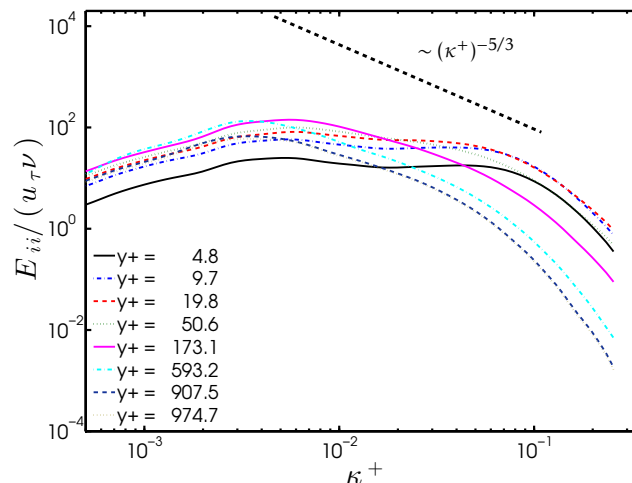
Figure 1.3 – Non-dimensional turbulent kinetic energy spectral density E/(\varepsilon \nu^5)^{1/4} at various y^+ locations at Re_\tau = 1000 .
