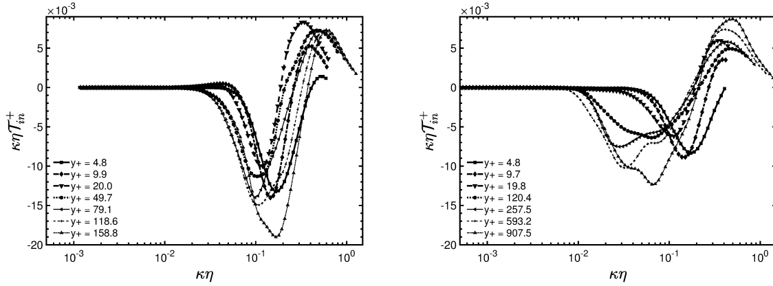
Figure 3.24 – In-plane nonlinear transfer spectral density, \kappa\eta T_{in}^+ , at various y^+ locations at Re_\tau = 180 and 1000 , respectively.
