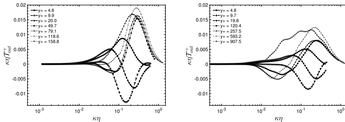
Figure 3.25 – Inter-plane nonlinear transfer spectral density, \kappa\eta\mathcal{T}_{out}^+ , at various y^+ locations at Re_\tau = 180 and 1000 , respectively.
