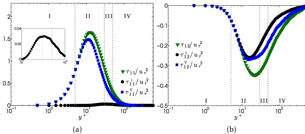
Figure 3.44 – Modeled and exact components of SGS stress tensor by applying: (a) Model I and (b) Model V.
