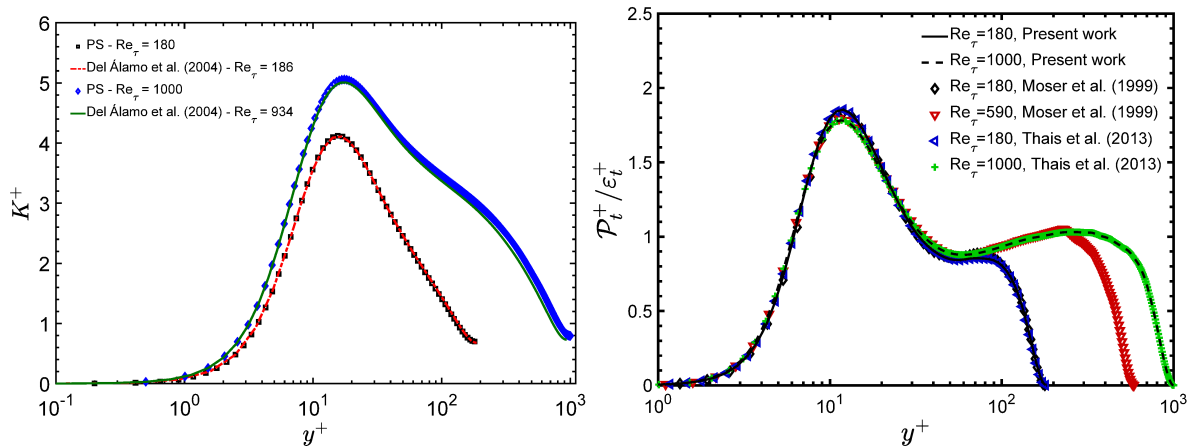
Figure 3.12 – Comparisons with results of Moser, Kim, and Mansour [117], Del Álamo et al. [37] and Thais, Mompean, and Gatski [147]: (a) Total turbulent kinetic energy dependence on the normalized distance from the wall and (b) ratio of production to dissipation of turbulent kinetic energy.
