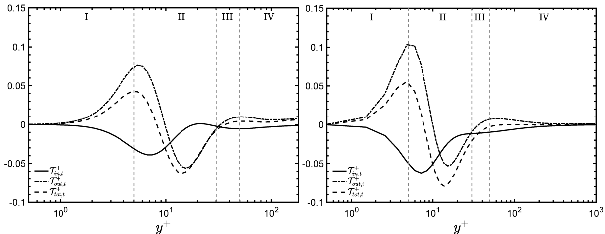
Figure 3.15 – In-plane, T_{in,t}^+ , and inter-plane, T_{out,t}^+ , nonlinear transfer contributions to the total nonlinear transfer, T_{tot,t}^+ , at Re_\tau = 180 and 1000 , respectively.
