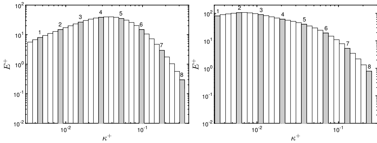
Figure 3.29 – Wavenumber bin distribution at y^+ \approx 40 and numeration plotted in Figs. 3.30-3.37 at Re_\tau = 180 and 1000 , respectively.
