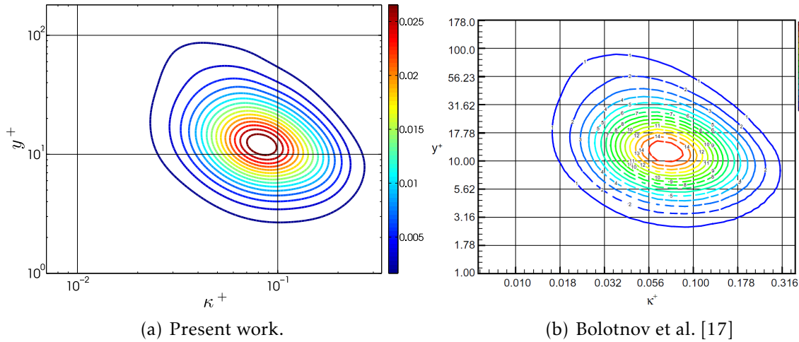
Figure B.3 – Comparison of turbulent production contour levels at Re_\tau = 180 .
